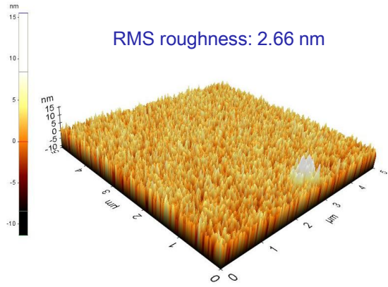
AFM image of Mo film (500nm) on glass
